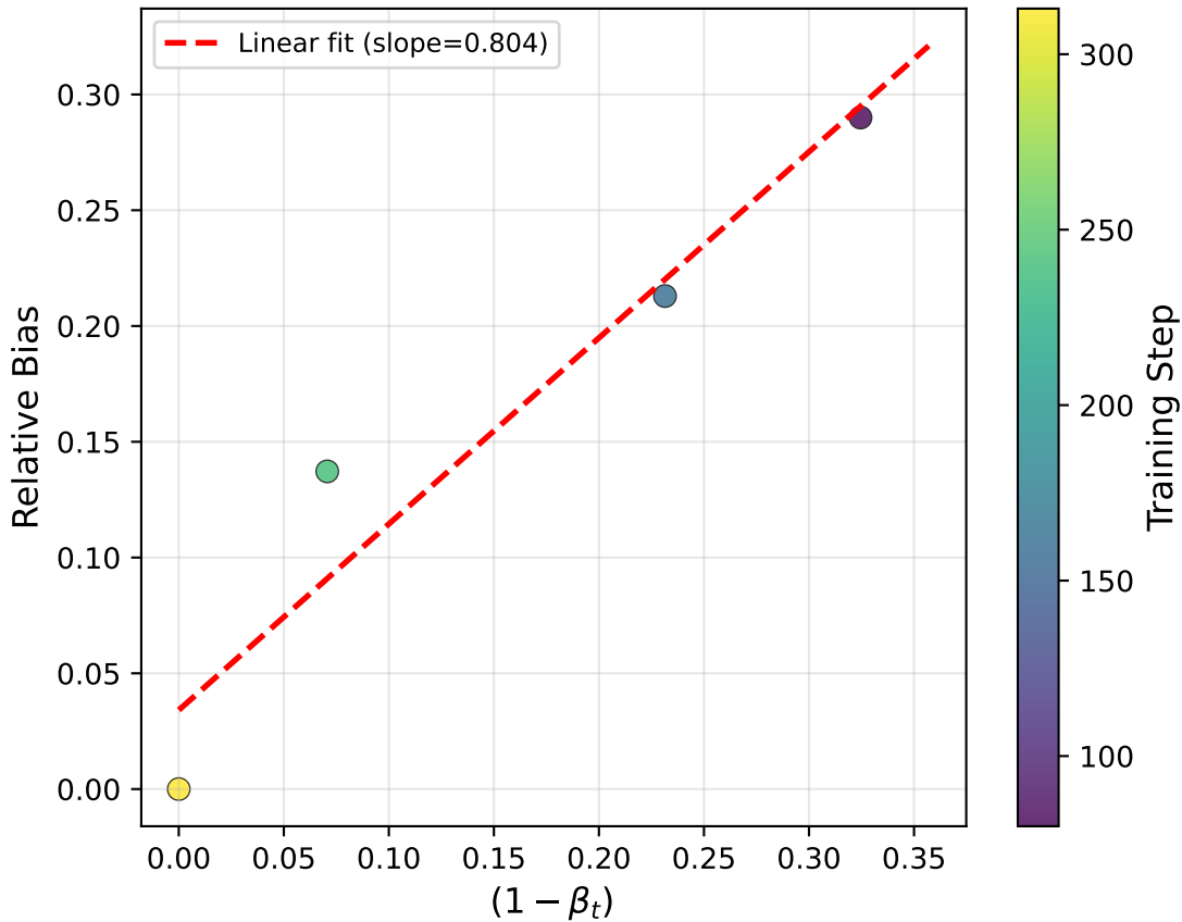
Qwen2.5-Math-7B: Bias \propto (1 - \beta_t)
